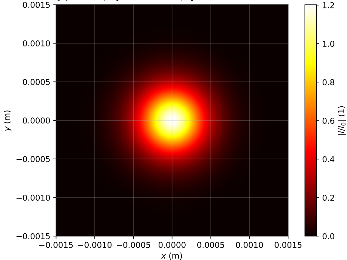
Intensity profile I(x, y, z = 0.716m)/I_0 , Pin=0.8Pcr, artificial time
